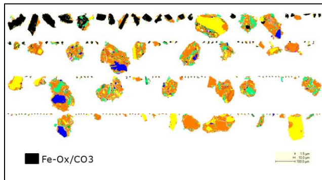
Qemscan analysis for sample at loadport in (upper) and sample at disport (lower). The latter indicates increased amount of magnetite potentially from adulteration of the samples prior to analysis.
